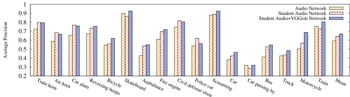
Figure 4: Average precision comparison on the 17 sound event classes of DCASE17 obtained by the conventional audio network, and our proposed student audio network trained with or without the pre-trained VGGish representation.
